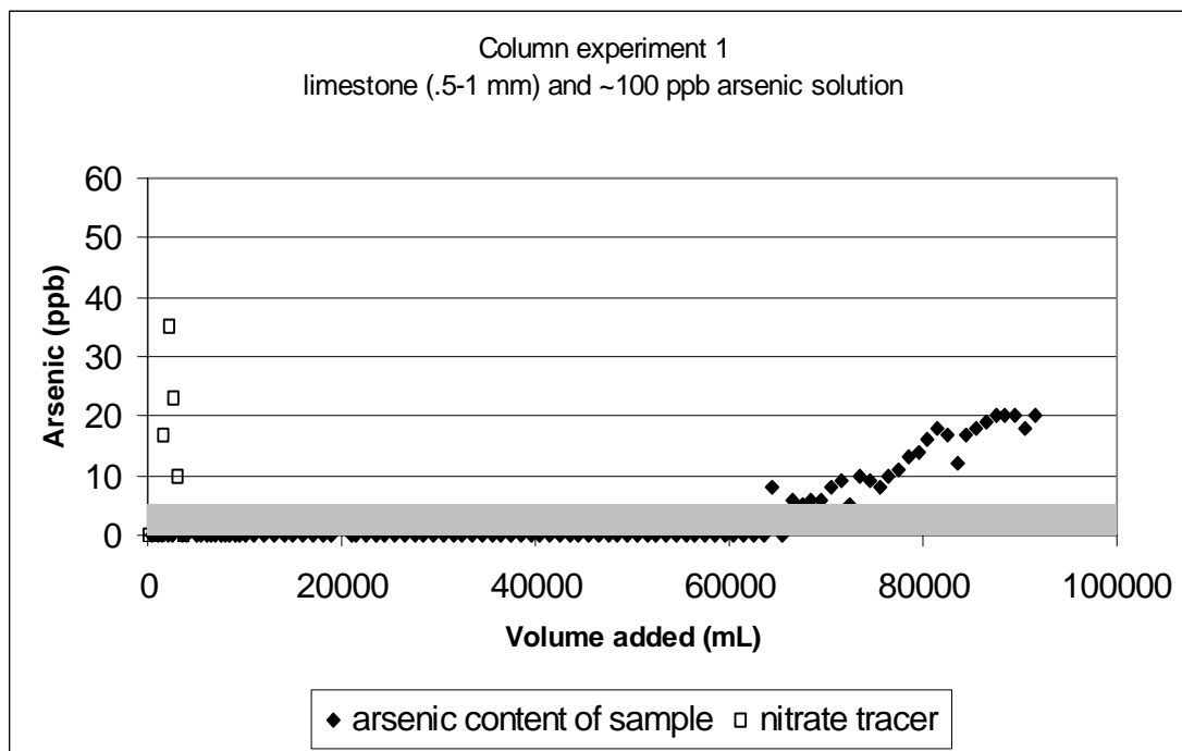
Figure 5. Graph of data from column experiment 1. Shaded area is BDL.
