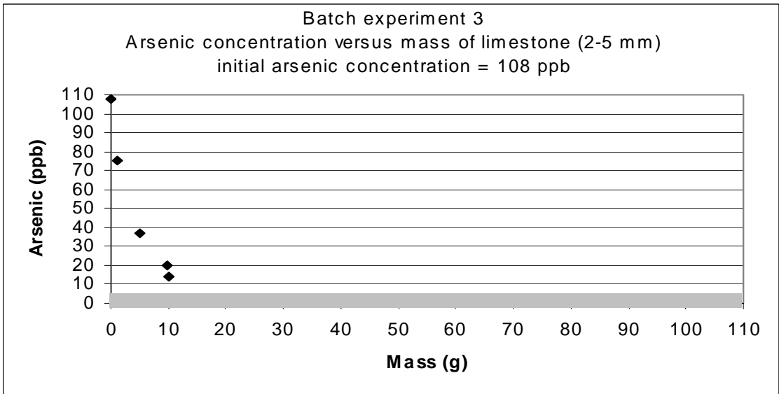
Figure 2. Graph of data from batch experiment 3. Shaded area is BDL.
