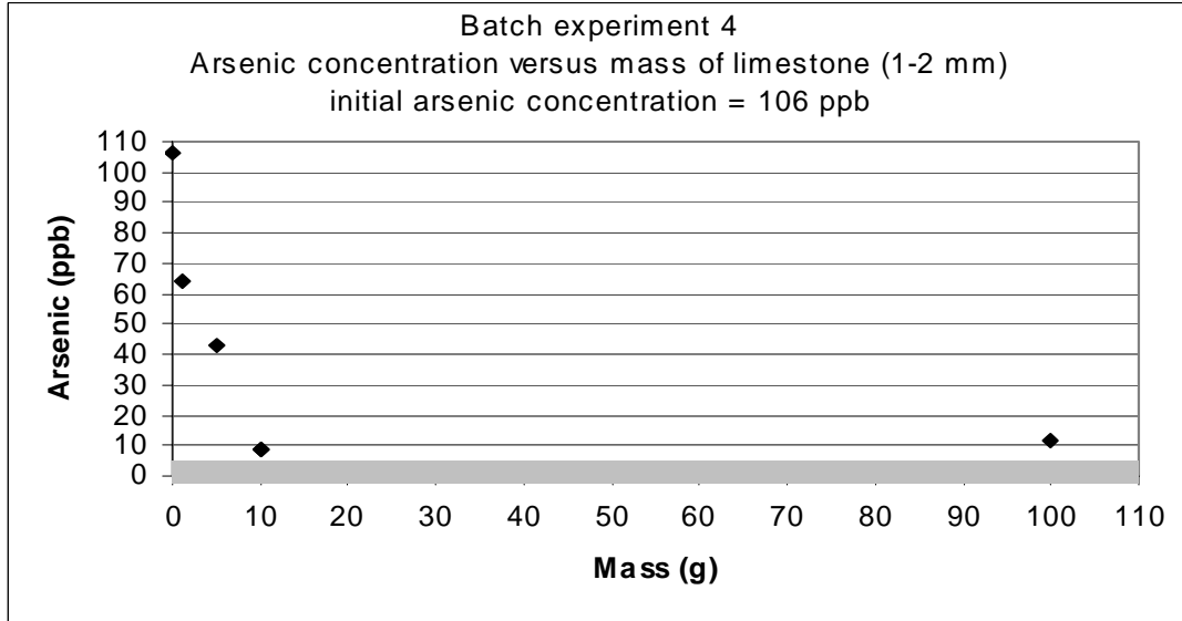
Figure 3. Graph of data from batch experiment 4. Shaded area is BDL.
